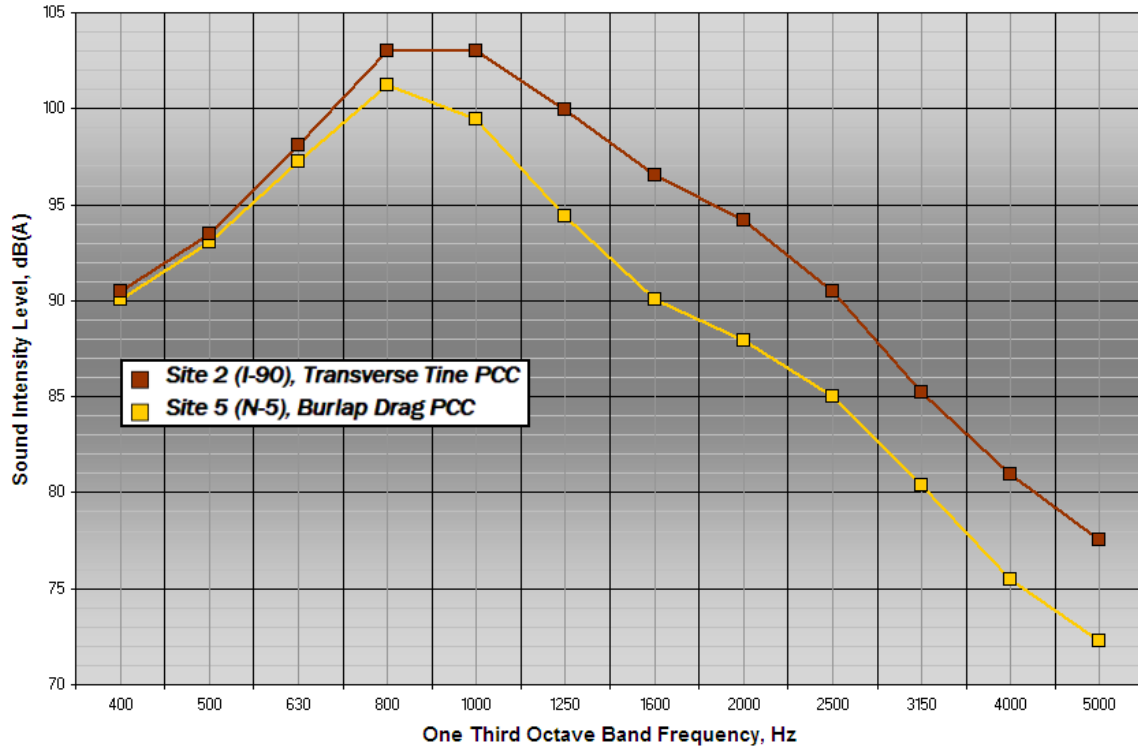
Figure 7. One-Third Octave Band Levels for Concrete Pavements
