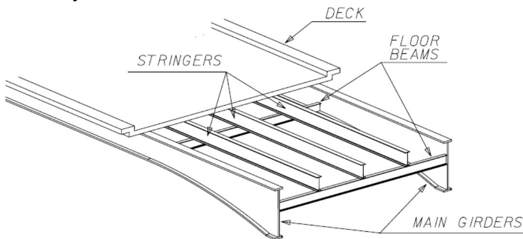
CROSS SECTION OF A TWO-GIRDER SYSTEM
