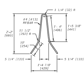
REBAR DETAIL LEFT END
