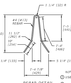
REBAR DETAIL
