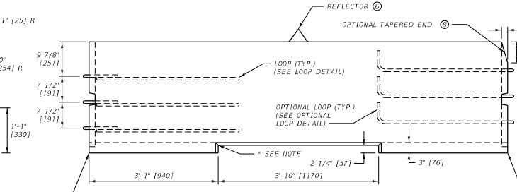
ELEVATION VIEW
