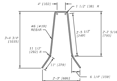
REBAR DETAIL
