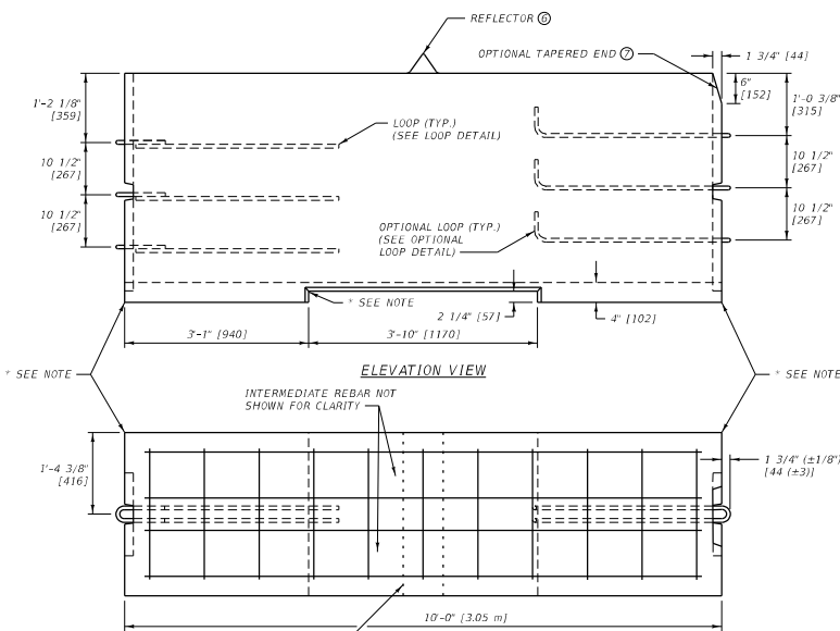
PLAN VIEW
