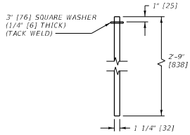
CONNECTING PIN DETAIL
