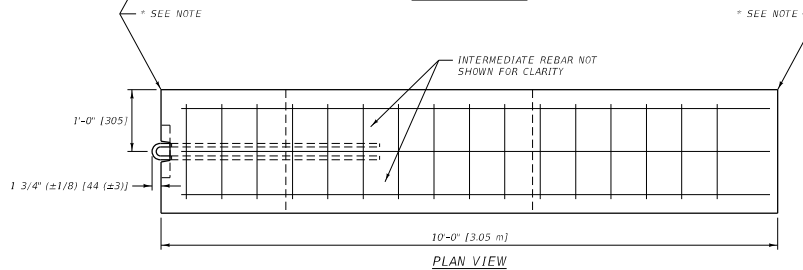
PLAN VIEW
