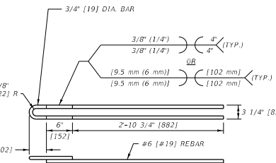
LOOP DETAIL
