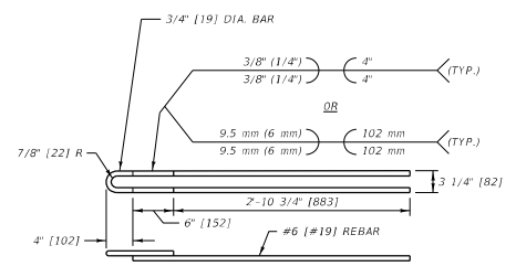
LOOP DETAIL
