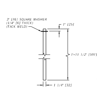
CONNECTING PIN DETAIL
