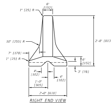
RIGHT END VIEW
