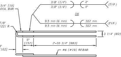
LOOP DETAIL
