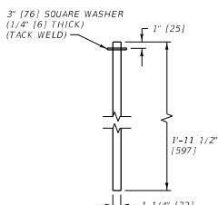
CONNECTING PIN DETAIL
