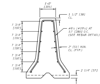
END VIEW
