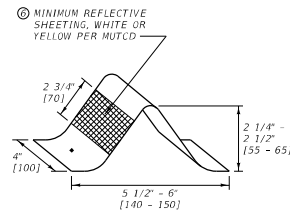
REFLECTOR (SEE NOTES)
