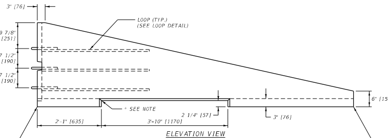
ELEVATION VIEW
