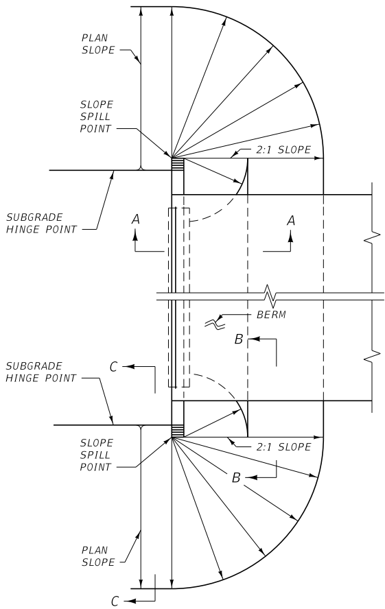
PLAN VIEW
