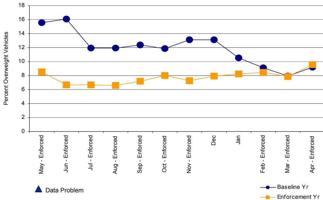
Figure B-3. Percent Overweight Commercial Vehicles by Month at the Stanford STARS Site, Baseline and Focused Enforcement Year
