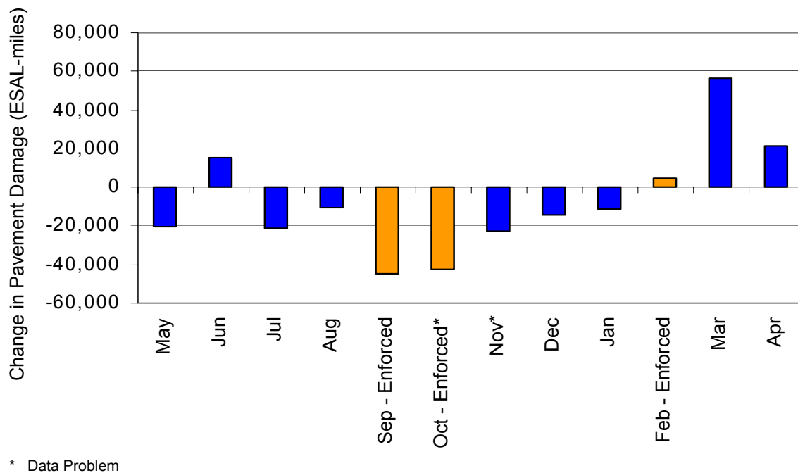
Figure D-6. Change in Pavement Damage for the Decker STARS Site, Baseline to Focused Enforcement Year
