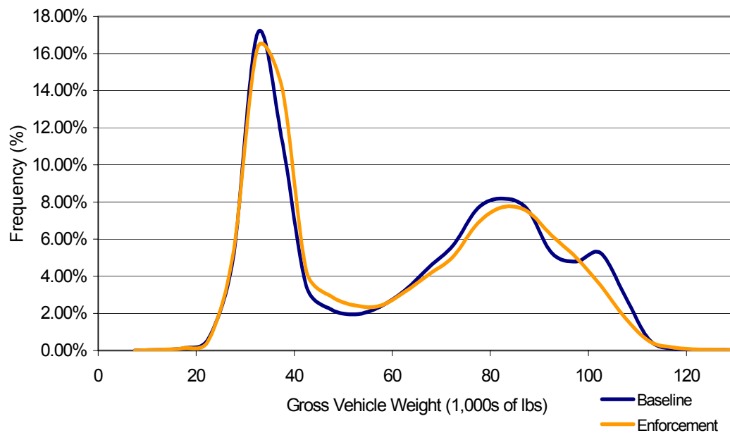
Figure C-11 Class 10 Gross Vehicle Weight Distributions at All STARS Sites not Selected for Focused Enforcement, Baseline and Focused Enforcement Year
