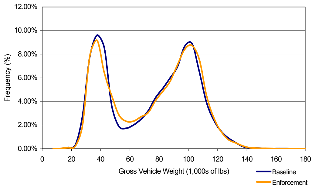
Figure C-12 Class 13 Gross Vehicle Weight Distributions at All STARS Sites not Selected for Focused Enforcement, Baseline and Focused Enforcement Year
