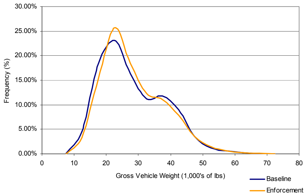
Figure C-9 Class 6 Gross Vehicle Weight Distributions at All STARS Sites not Selected for Focused Enforcement , Baseline and Focused Enforcement Year
