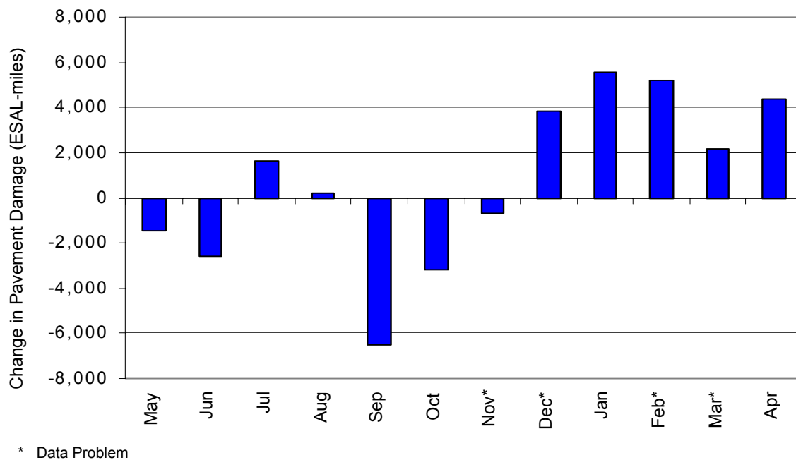
Figure D-16. Change in Pavement Damage for the Paradise STARS Site, Baseline to Focused Enforcement Year
