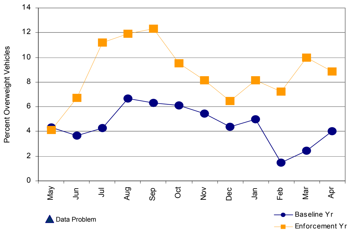
Figure B-10. Percent Overweight Commercial Vehicles by Month at the Broadview STARS Site, Baseline and Focused Enforcement Year
