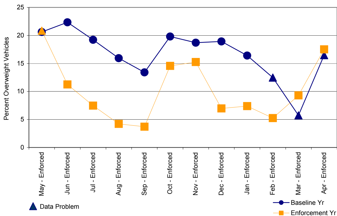
Figure B-1. Percent Overweight Commercial Vehicles by Month at the Four Corners/Gallatin STARS Site , Baseline and Focused Enforcement Year
