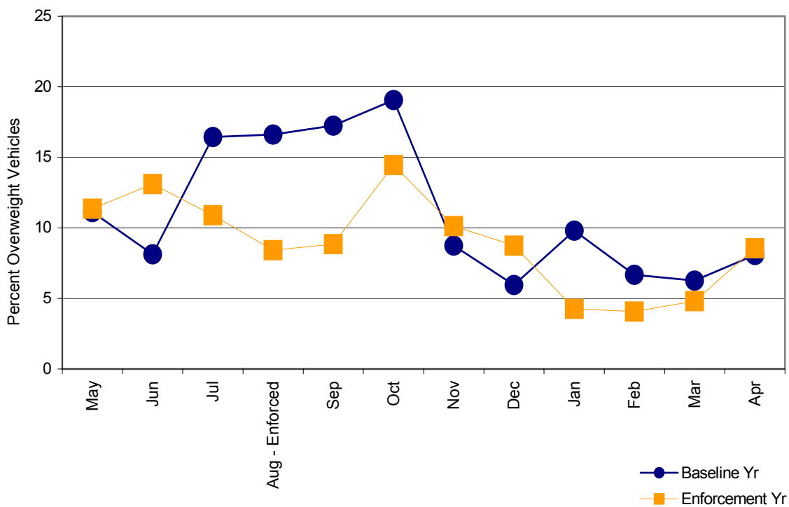
Figure B-8. Percent Overweight Commercial Vehicles by Month at the Miles City East STARS Site, Baseline and Focused Enforcement Year
