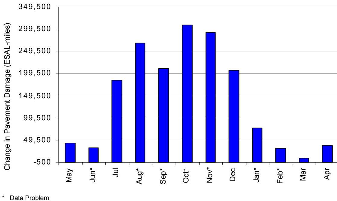
Figure D-12. Change in Pavement Damage for the Fort Benton STARS Site, Baseline to Focused Enforcement Year
