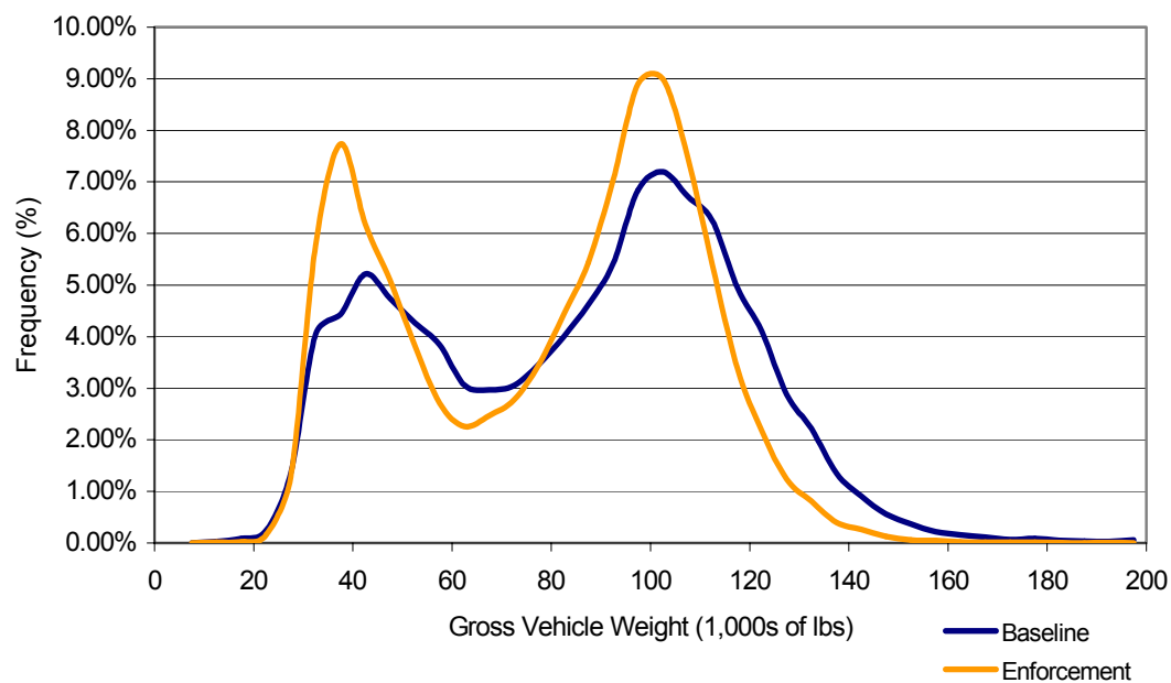
Figure C-4. Class 13 Gross Vehicle Weight Distributions at All STARS Sites with More than Six Months of Focused Enforcement , Baseline and Focused Enforcement Year
