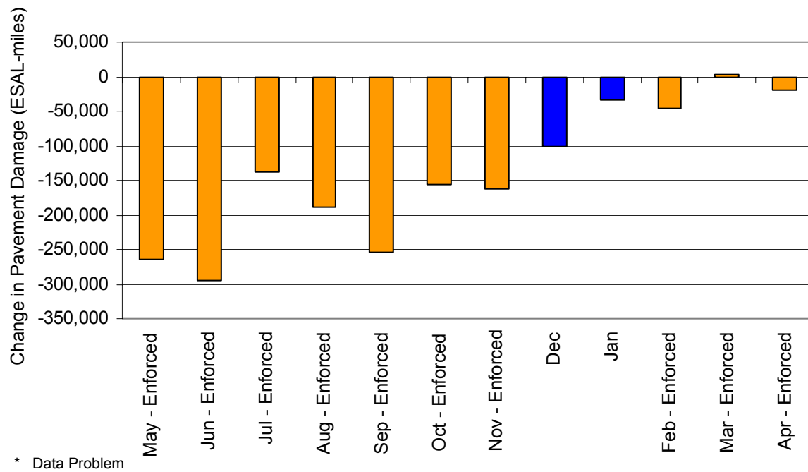
Figure D-3. Change in Pavement Damage for the Stanford STARS Site, Baseline to Focused Enforcement Year
