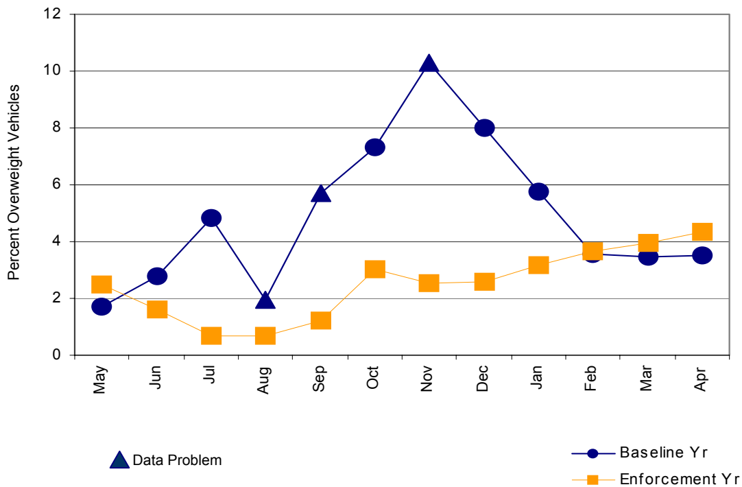
Figure B-14. Percent Overweight Commercial Vehicles by Month at the Havre East STARS Site, Baseline and Focused Enforcement Year
