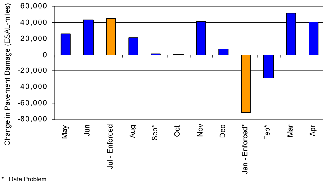
Figure D-5. Change in Pavement Damage for the Arlee STARS Site, Baseline to Focused Enforcement Year
