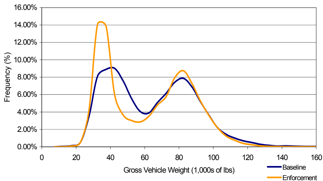
Figure C-3. Class 10 Gross Vehicle Weight Distributions at All STARS Sites with More than Six Months of Focused Enforcement , Baseline and Focused Enforcement Year
