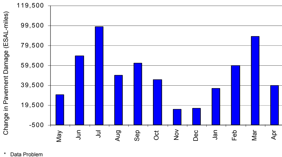
Figure D-10. Change in Pavement Damage for the Broadview STARS Site, Baseline to Focused Enforcement Year
