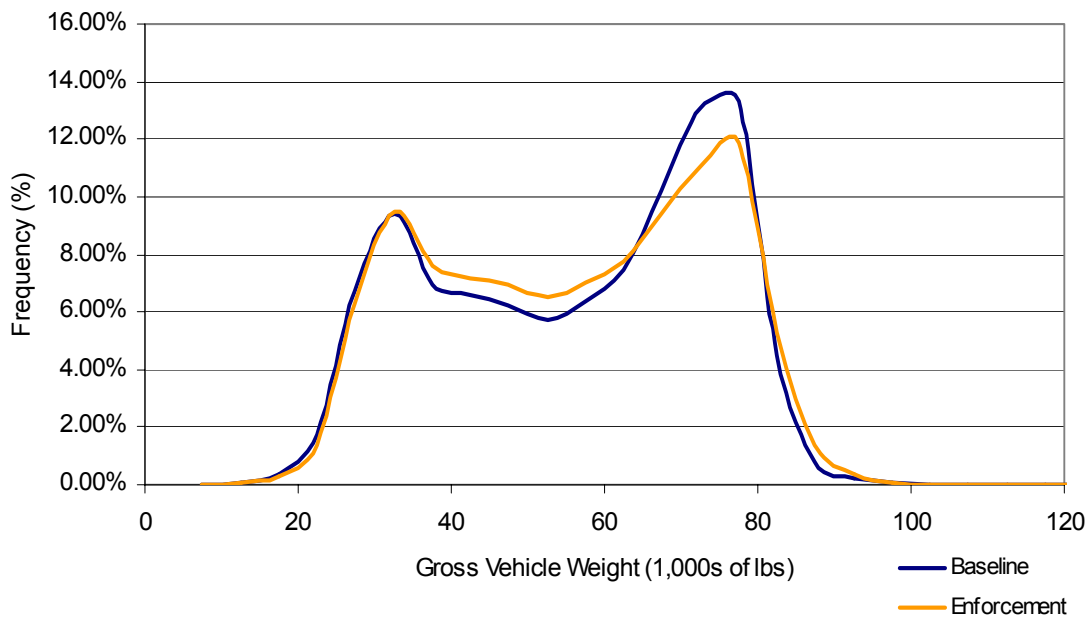
Figure C-10 Class 9 Gross Vehicle Weight Distributions at All STARS Sites not Selected for Focused Enforcement , Baseline and Focused Enforcement Year
