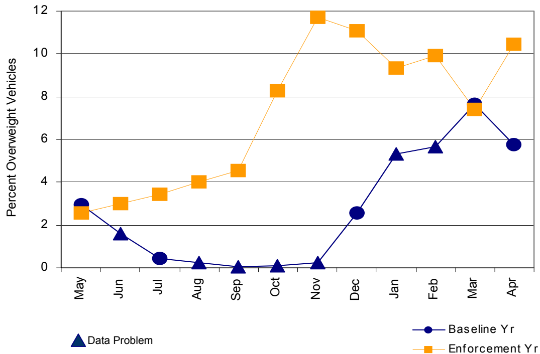
Figure B-12. Percent Overweight Commercial Vehicles by Month at the Fort Benton STARS Site, Baseline and Focused Enforcement Year
