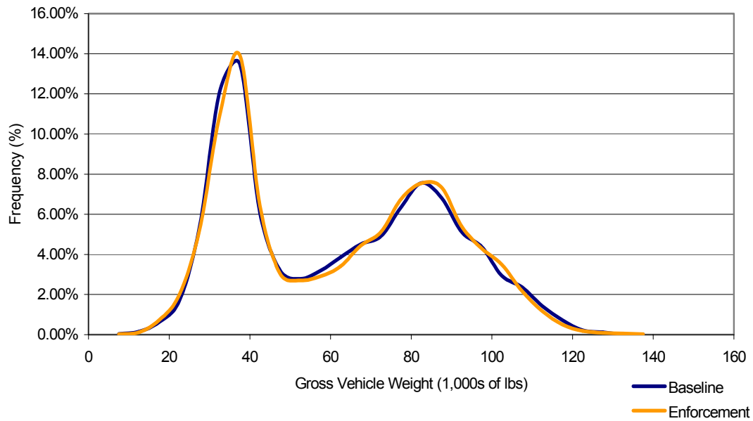
Figure C-7 Class 10 Gross Vehicle Weight Distributions at All STARS Sites with One to Six Months of Focused Enforcement, Baseline and Focused Enforcement Year
