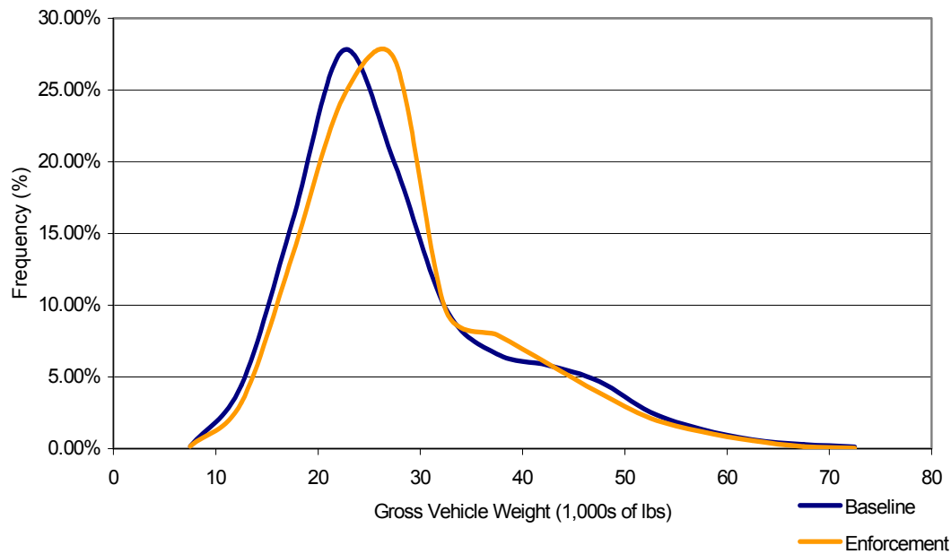
Figure C-5 Class 6 Gross Vehicle Weight Distributions at All STARS Sites with One to Six Months of Focused Enforcement, Baseline and Focused Enforcement Year
