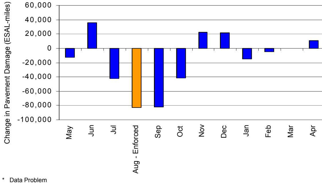
Figure D-8. Change in Pavement Damage for the Miles City East STARS Site, Baseline to Focused Enforcement Year
