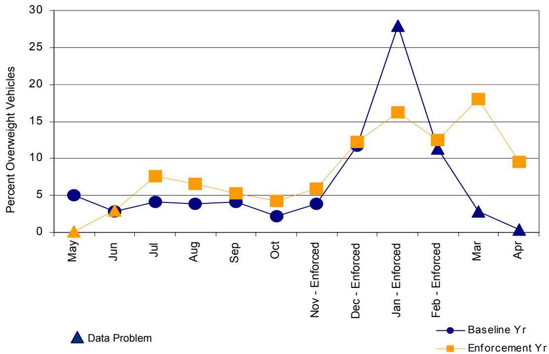
Figure B-9. Percent Overweight Commercial Vehicles by Month at the Ulm STARS Site, Baseline and Focused Enforcement Year
