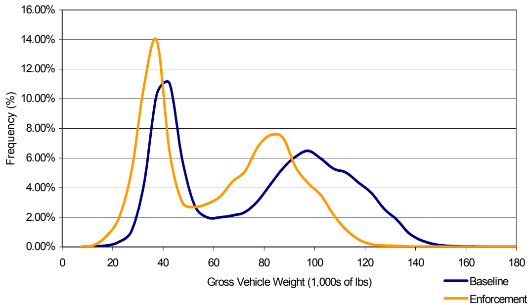
Figure C-8 Class 13 Gross Vehicle Weight Distributions at All STARS Sites with One to Six Months of Focused Enforcement, Baseline and Focused Enforcement Year
