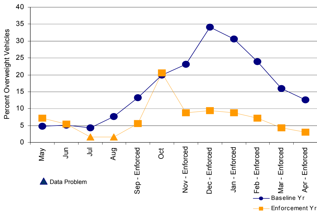
Figure B-2. Percent Overweight Commercial Vehicles by Month at the Ryegate STARS Site , Baseline and Focused Enforcement Year
