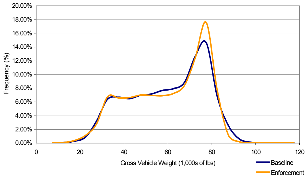
Figure C-6 Class 9 Gross Vehicle Weight Distributions at All STARS Sites with One to Six Months of Focused Enforcement, Baseline and Focused Enforcement Year
