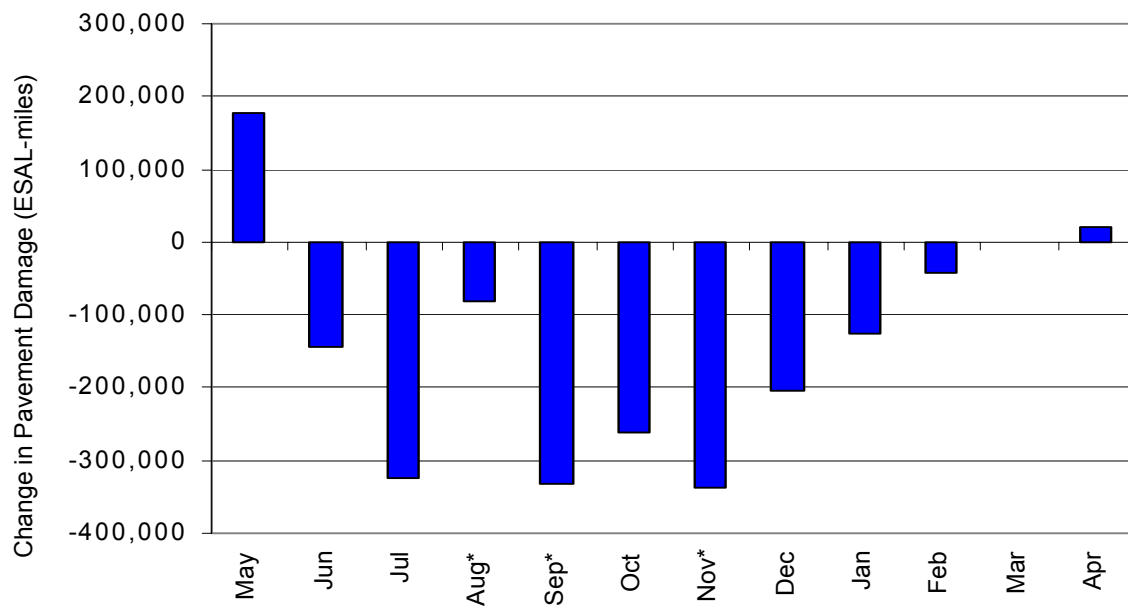
Figure D-13. Change in Pavement Damage for the Galen STARS Site, Baseline to Focused Enforcement Year
