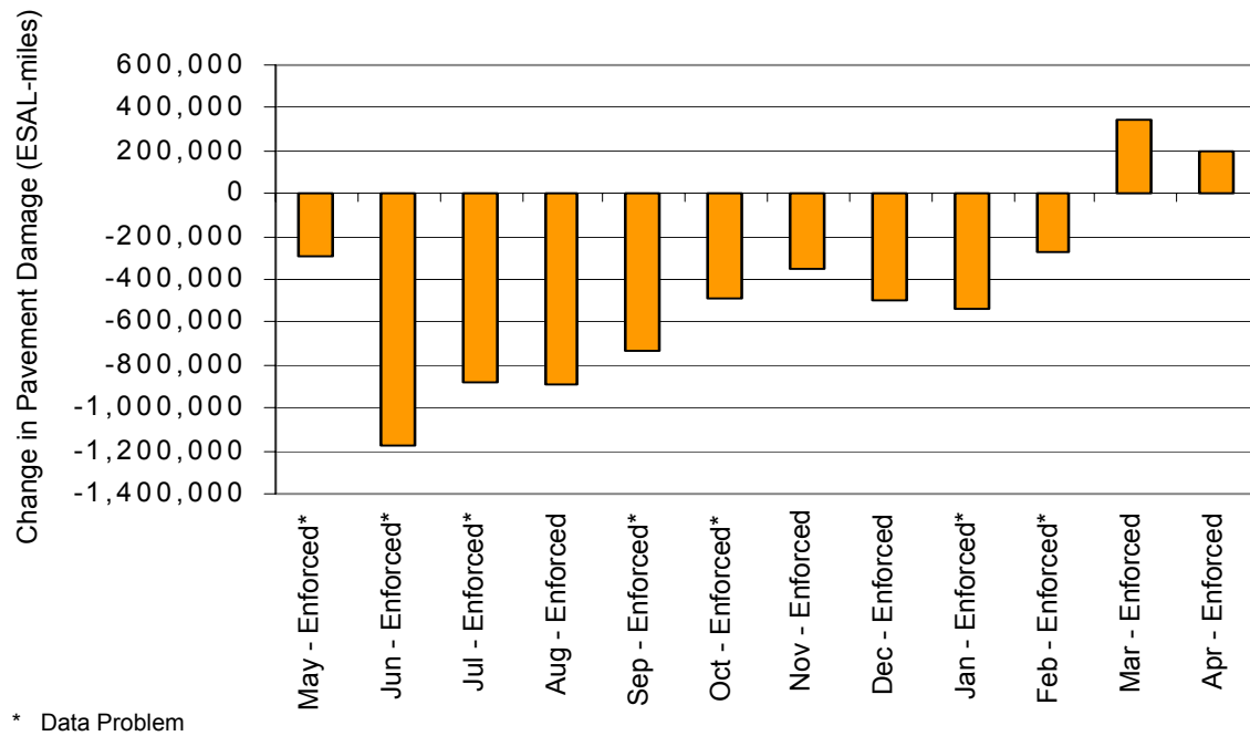
Figure D-1. Change in Pavement Damage for the Four Corners/Gallatin STARS Site, Baseline to Focused Enforcement Year
