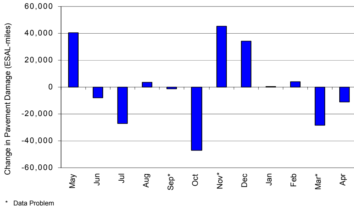
Figure D-11. Change in Pavement Damage for the Culbertson STARS Site, Baseline to Focused Enforcement Year
