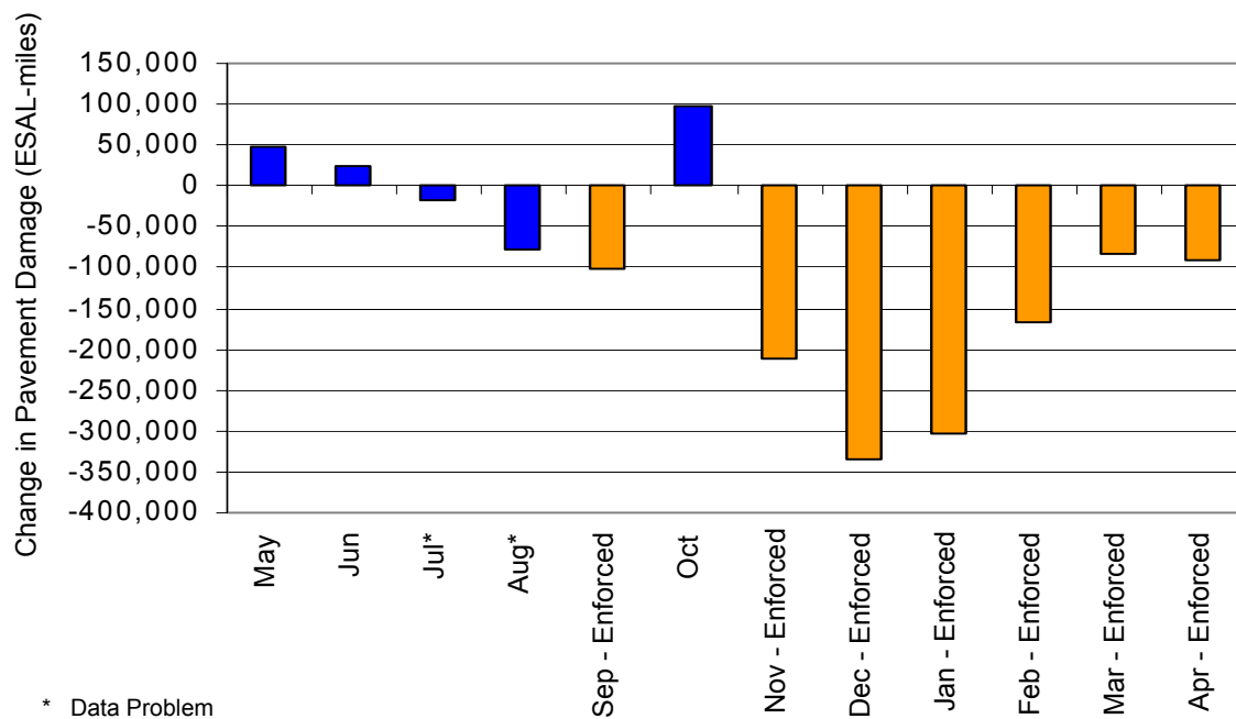
Figure D-2. Change in Pavement Damage for the Ryegate STARS Site, Baseline to Focused Enforcement Year
