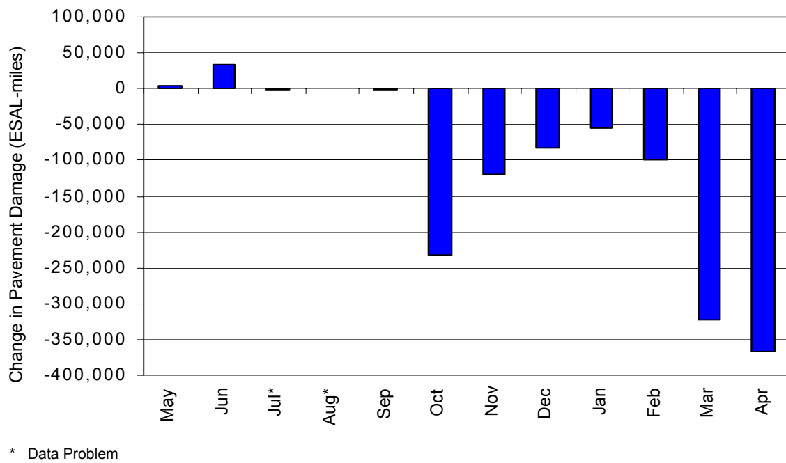
Figure D-15. Change in Pavement Damage for the Lima STARS Site, Baseline to Focused Enforcement Year
