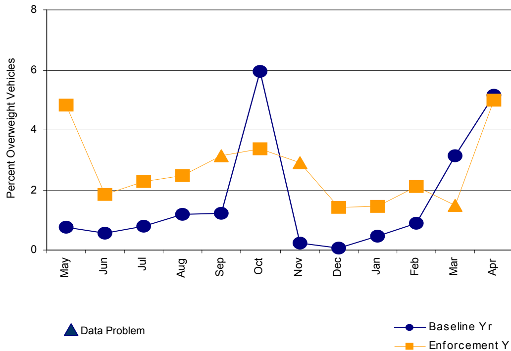
Figure B-11. Percent Overweight Commercial Vehicles by Month at the Culbertson STARS Site, Baseline and Focused Enforcement Year
