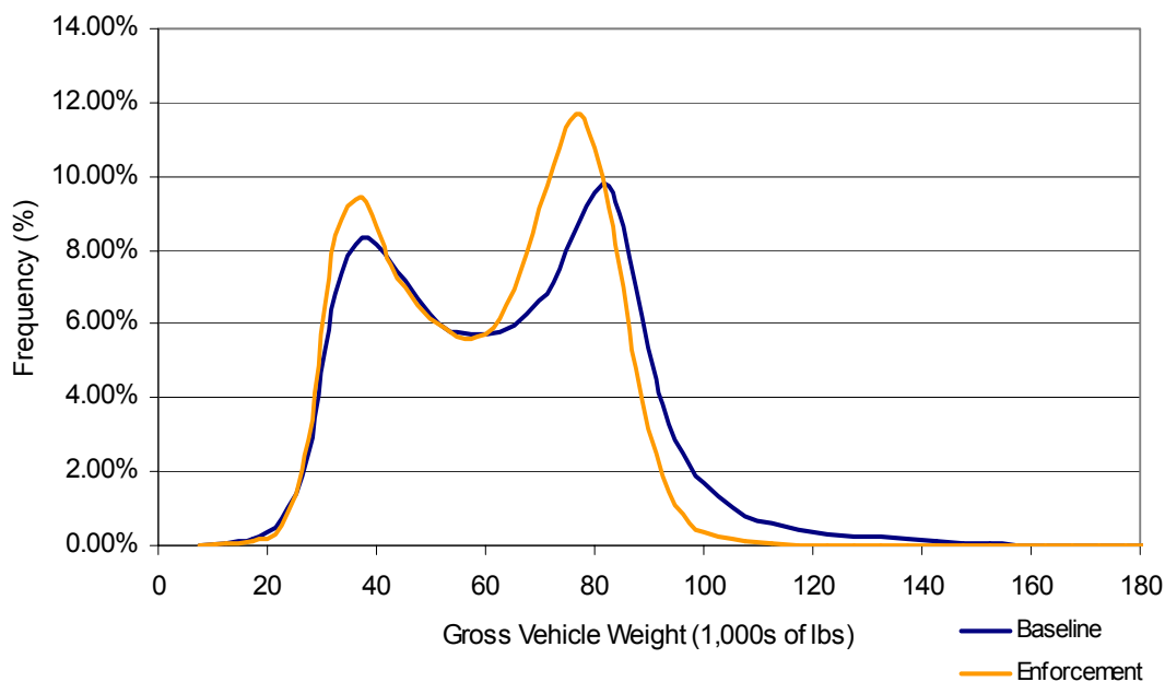
Figure C-2. Class 9 Gross Vehicle Weight Distributions at All STARS Sites with More than Six Months of Focused Enforcement, Baseline and Focused Enforcement Year
