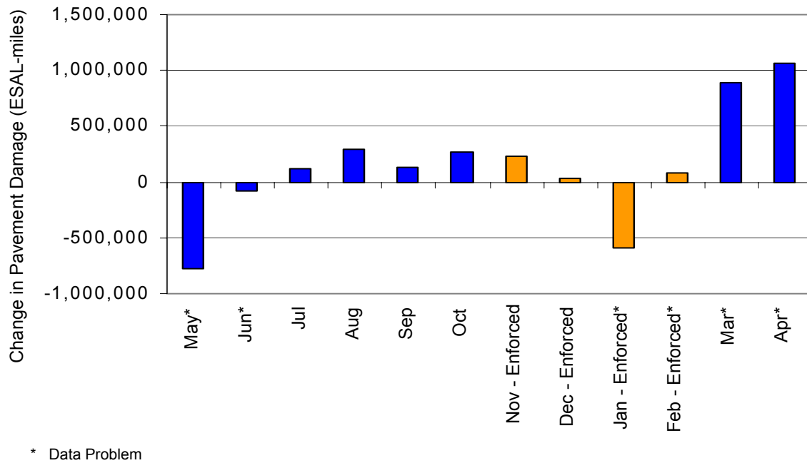
Figure D-9. Change in Pavement Damage for the Ulm STARS Site, Baseline to Focused Enforcement Year
