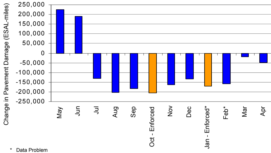
Figure D-7. Change in Pavement Damage for the Manhattan STARS Site, Baseline to Focused Enforcement Year
