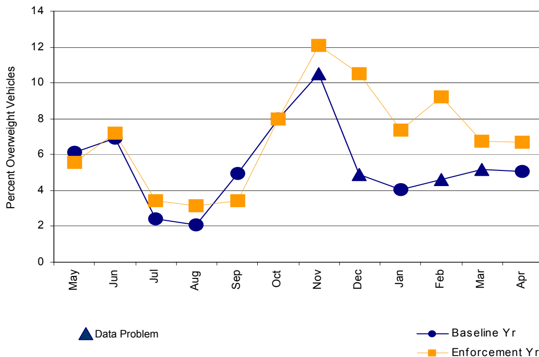
Figure B-16. Percent Overweight Commercial Vehicles by Month at the Paradise STARS Site, Baseline and Focused Enforcement Year
