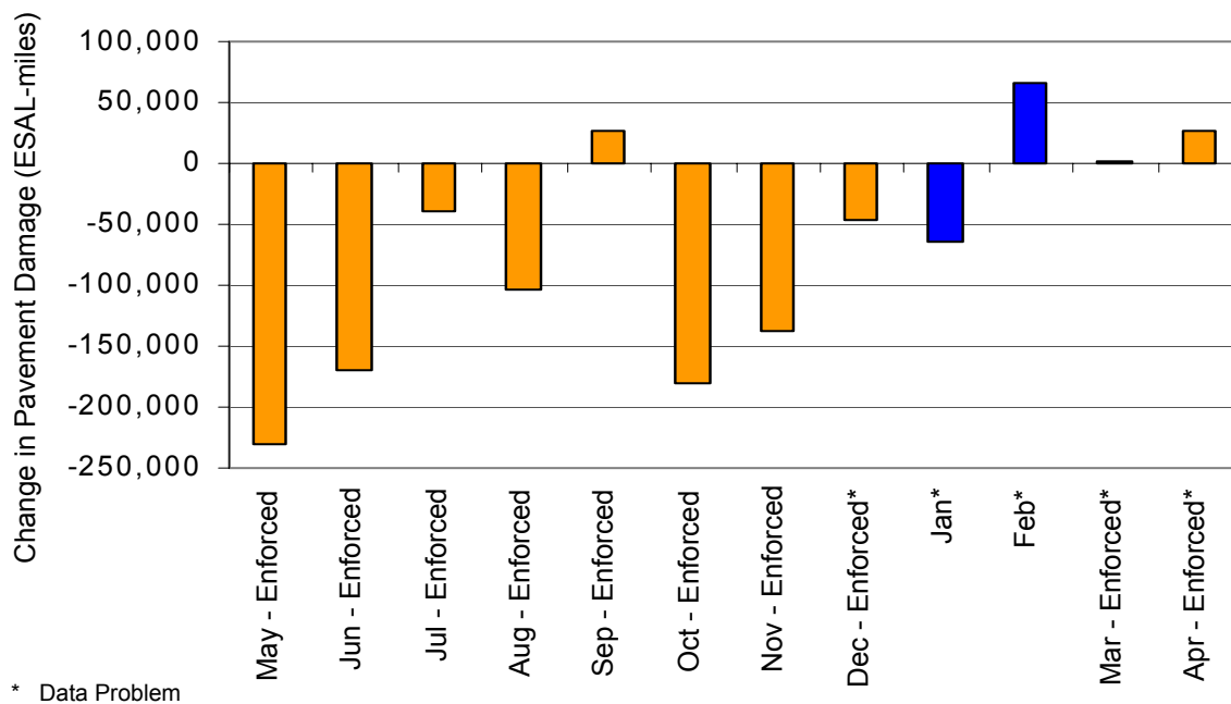
Figure D-4. Change in Pavement Damage for the Townsend STARS Site, Baseline to Focused Enforcement Year
