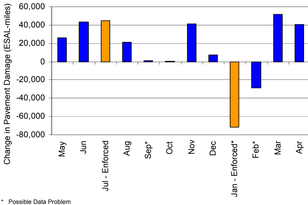
Figure 3-17. Change in Pavement Damage for the Arlee STARS Site, Baseline to Focused Enforcement Year
