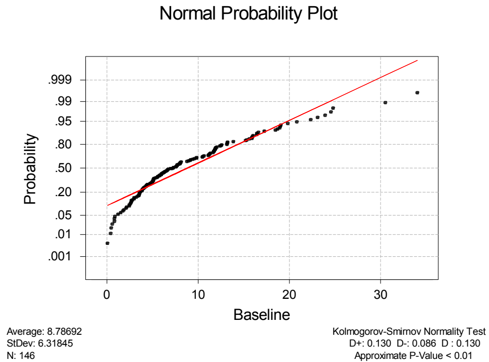
Figure 3-7. Percentage of Overweight Vehicles Normality Plot, Baseline Year
