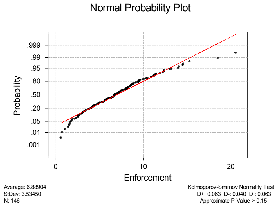
Figure 3-8. Percentage of Overweight Vehicles Normality Plot, Focused Enforcement Year
