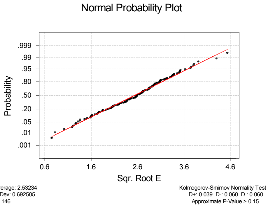
Figure 3-10. Square Root-transformed Percentage of Overweight Vehicles Normality Plot, Focused Enforcement Year
