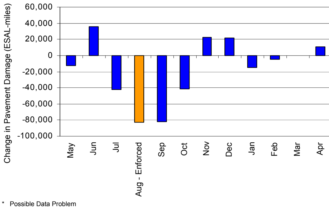
Figure 3-18. Change in Pavement Damage for the Miles City East STARS Site, Baseline to Focused Enforcement Year
