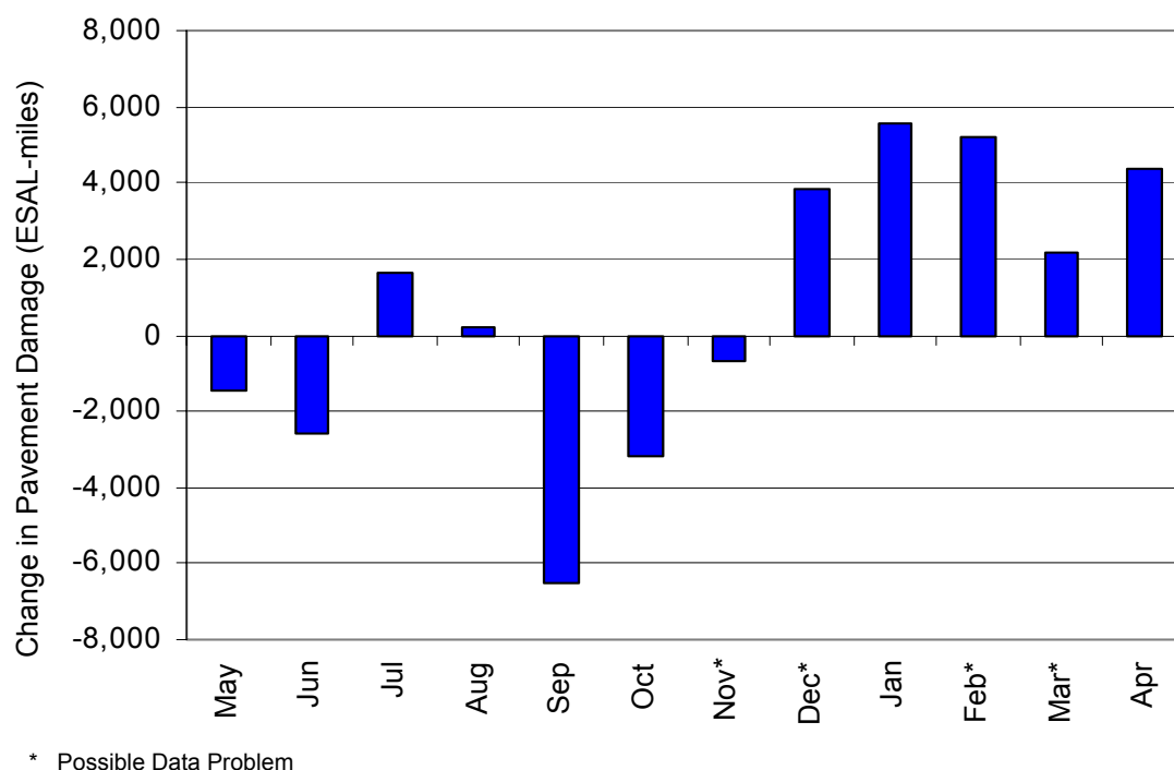
Figure 3-20. Change in Pavement Damage for the Paradise STARS Site, Baseline to Focused Enforcement Year
